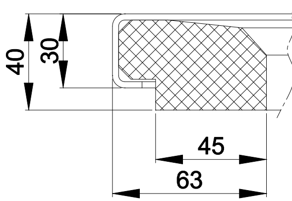
Detail A M5:1
